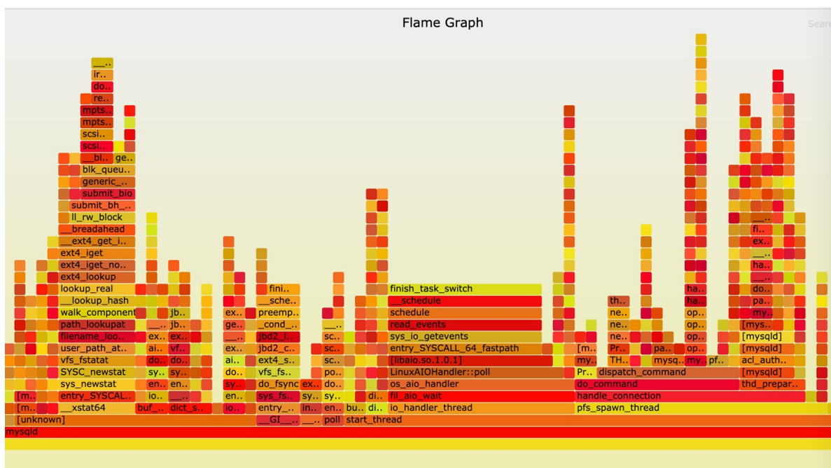
Figure 7-7. MySQL flame graph
