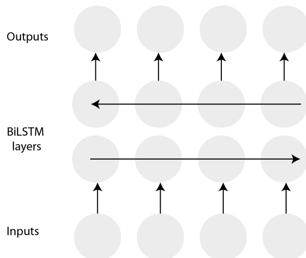
Figure 5-5. A biLSTM
