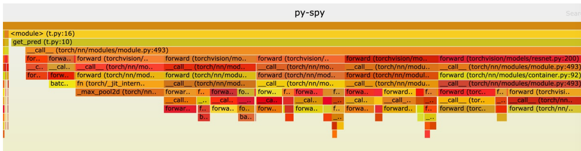
Figure 7-8. Flame graph on ResNet loading and inference
